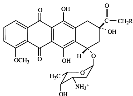
Figure 1. Chemical structure of doxorubicin hydrochloride. R = OH.
